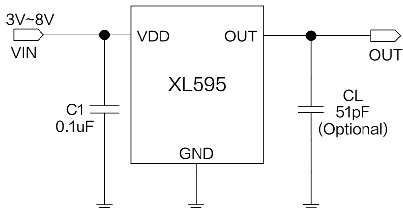
Figure1. XL595 Typical application schematic
