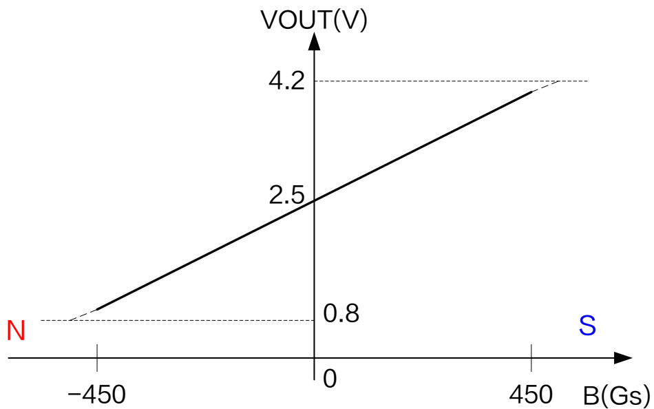
Figure4. XL595 Output characteristic curve
