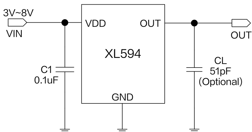
Figure1. XL594 Typical application schematic
