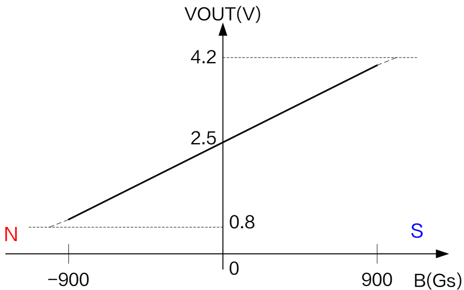
Figure4. XL594 Output characteristic curve
