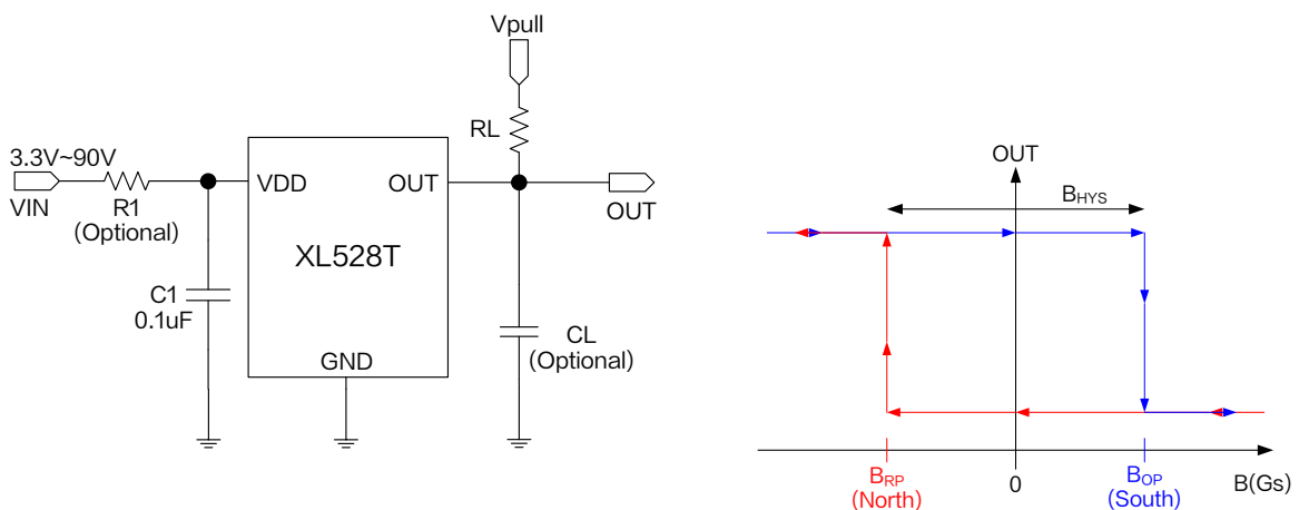
Figure1.XL528T Typical application schematic and output characteristic curve
