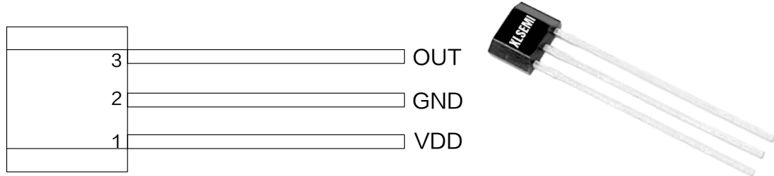
Figure2.Pin Configuration of XL528T
