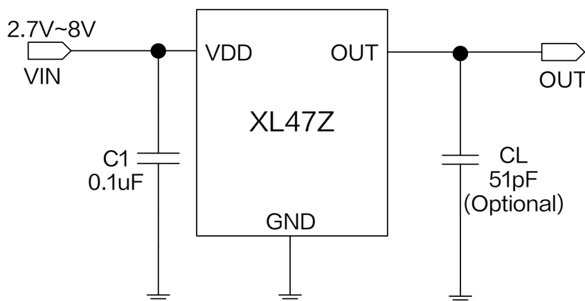
Figure1.XL47Z Typical application schematic
