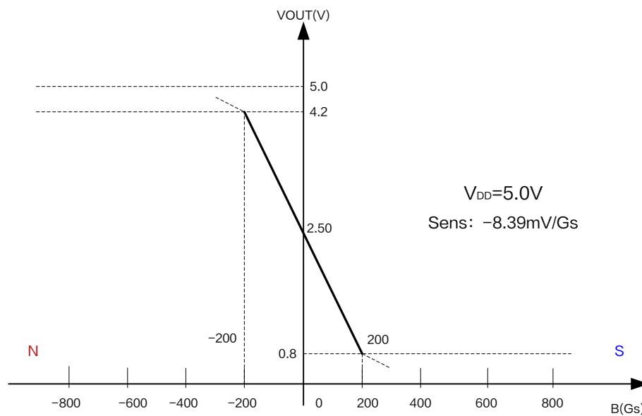
Figure6.XL47Z Output characteristic curve ( V_{DD} = 5.0V )
