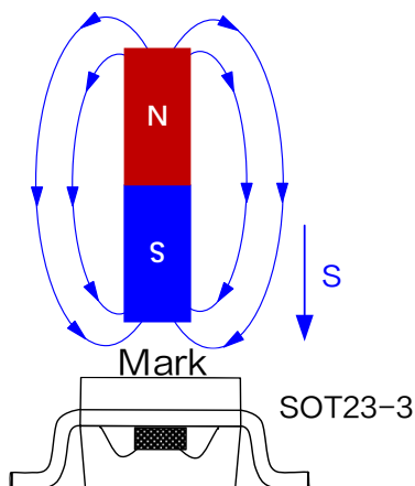
Figure4.Test Schematic of XL47Z
