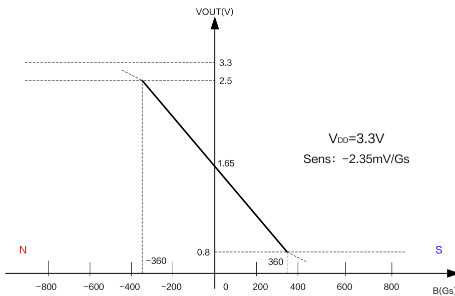
Figure5.XL47Z Output characteristic curve ( V_{DD} = 3.3\text{V} )
