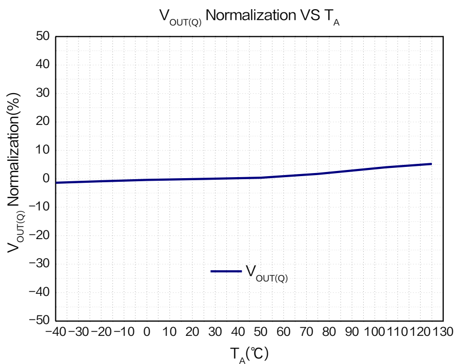
Figure 9. Static output voltage versus temperature curve of XL47E ( V_{DD} = 5.0V )
