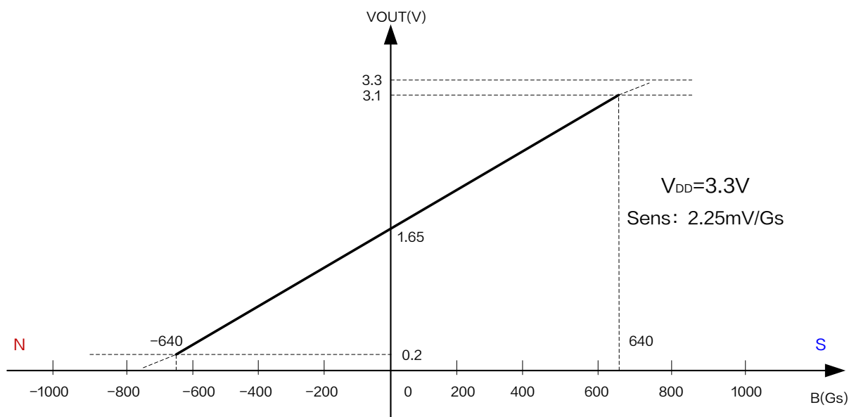
Figure5. Output Characteristic Curve of XL46T ( V_{DD}=3.3\text{V} )
