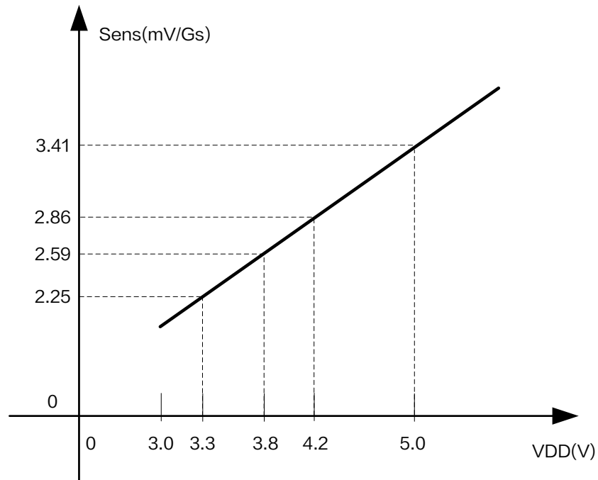
Figure6. Sensitivity Linear Curve of XL46T
