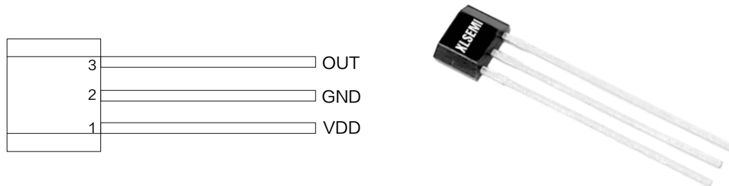
Figure2. Pin Configuration of XL46T
