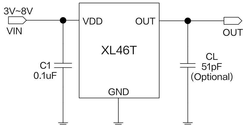
Figure1. XL46T Typical application schematic
