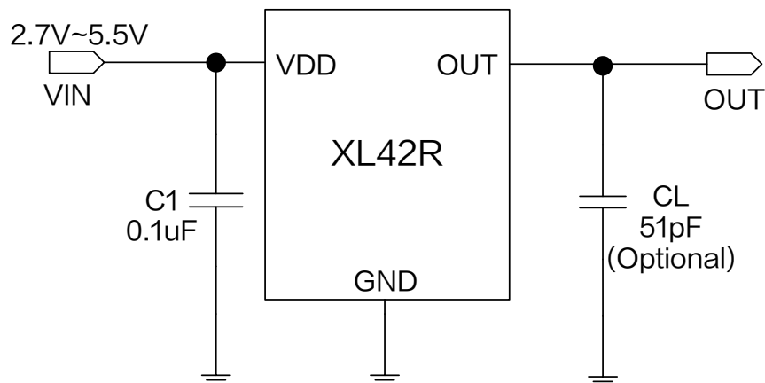
Figure1.XL42R Typical application schematic
