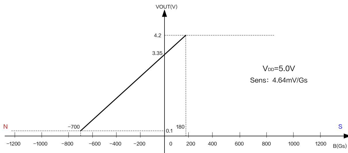
Figure6.XL42R Output characteristic curve ( V_{DD} = 5.0V )
