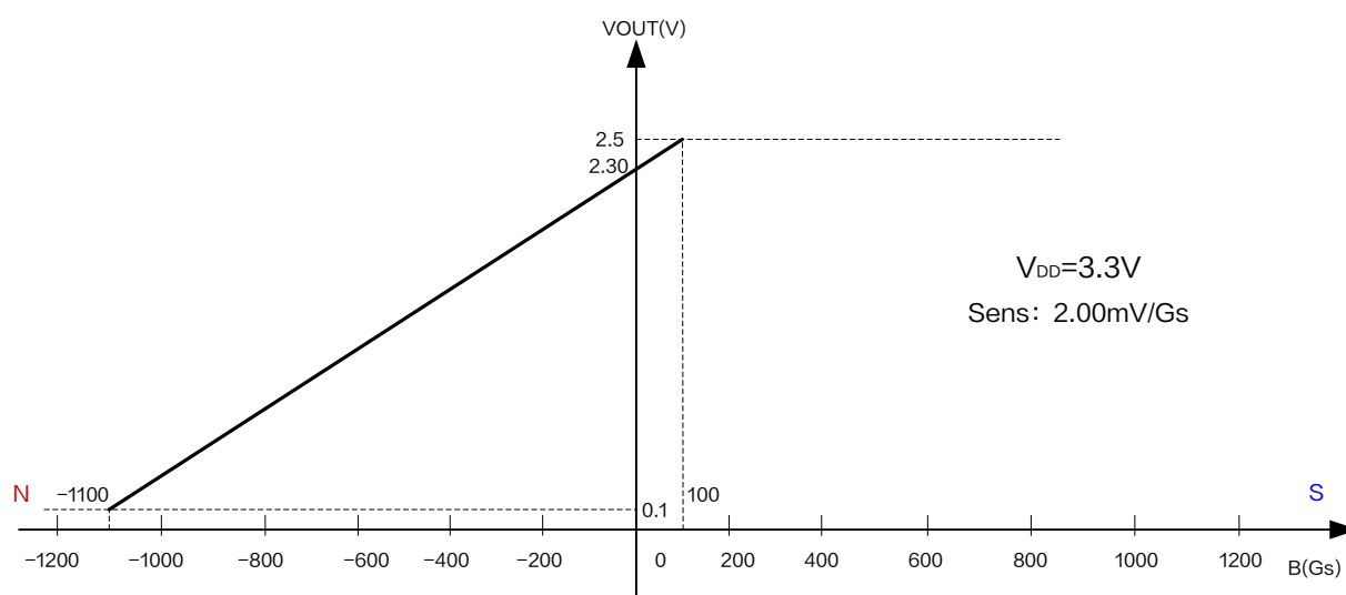
Figure5.XL42R Output characteristic curve ( V_{DD} = 3.3\text{V} )
