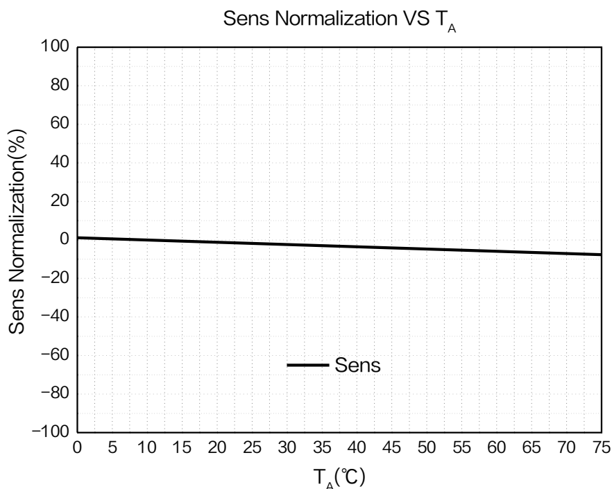
Figure7.Sensitivity versus temperature curve of XL42R ( V_{DD} = 3.3V )
