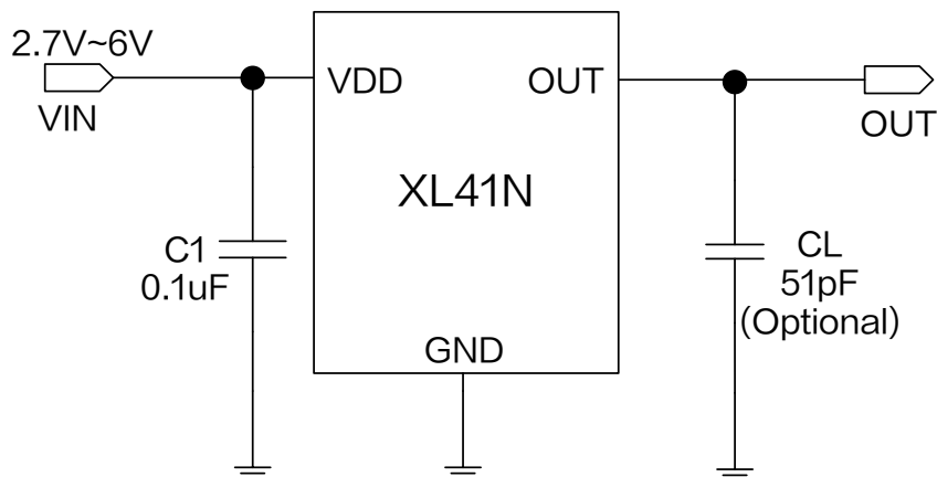
Figure1.XL41N Typical application schematic
