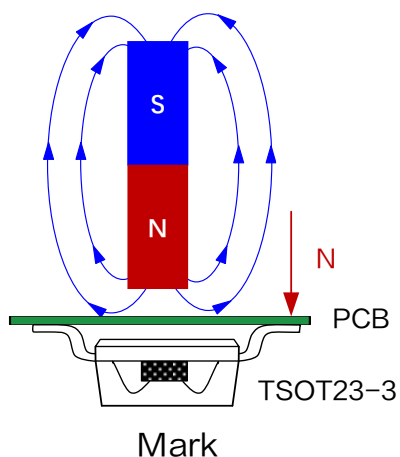
Figure4.Application diagram of XL41N
