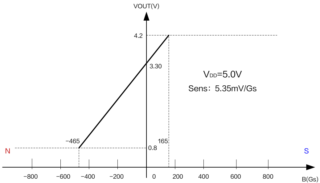
Figure6.XL41N Output characteristic curve ( V_{DD} = 5.0V )
