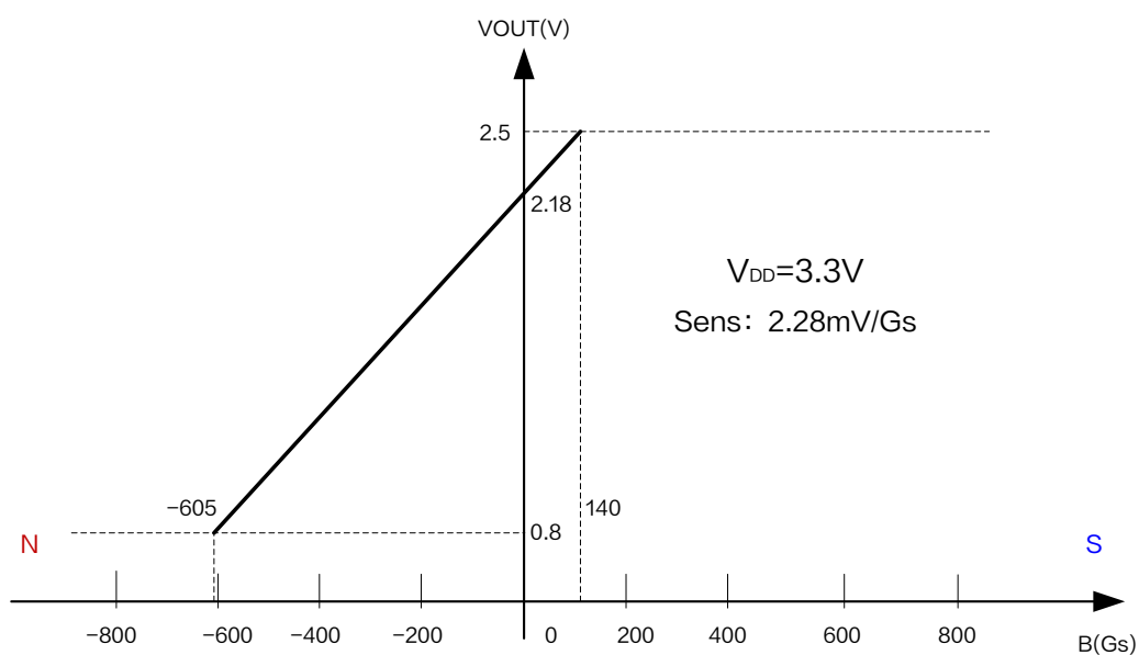
Figure5.XL41N Output characteristic curve ( V_{DD} = 3.3\text{V} )
