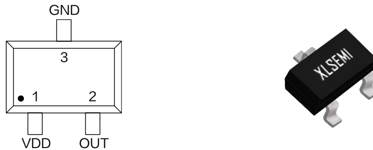
Figure2.Pin Configuration of XL41N
