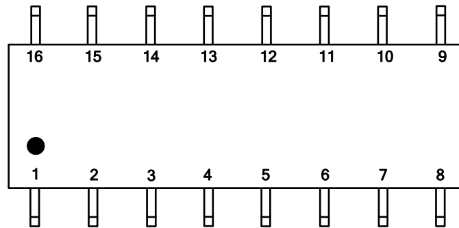
Figure2. Pin Configuration of XL1192 (Top View)
