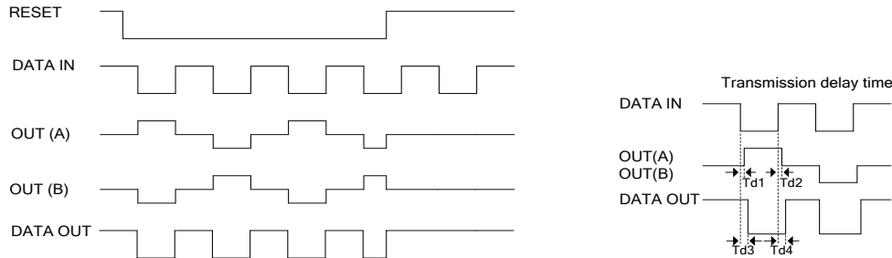
Figure5.XL1161 Timing Chart
