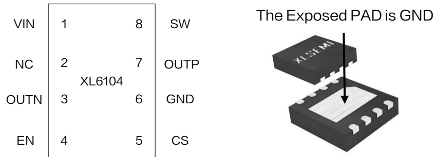
Figure2. Pin Configuration of XL6104
