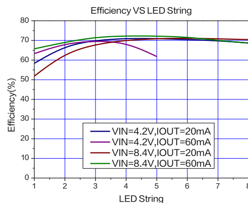
Figure7. XL6104 System Application and efficiency curve
