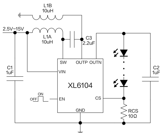
Figure7. XL6104 System Application and efficiency curve
