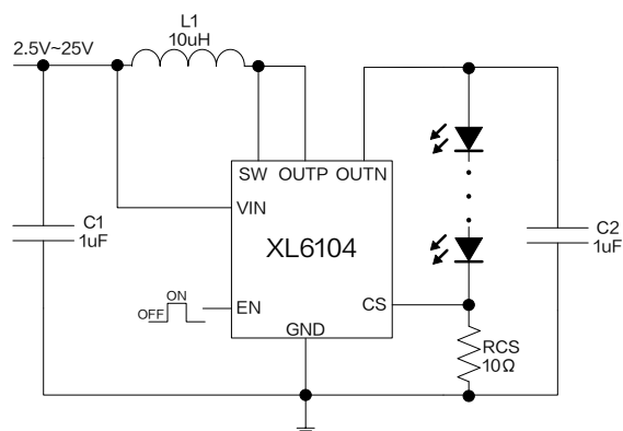
Figure6. XL6104 System Application and efficiency curve
