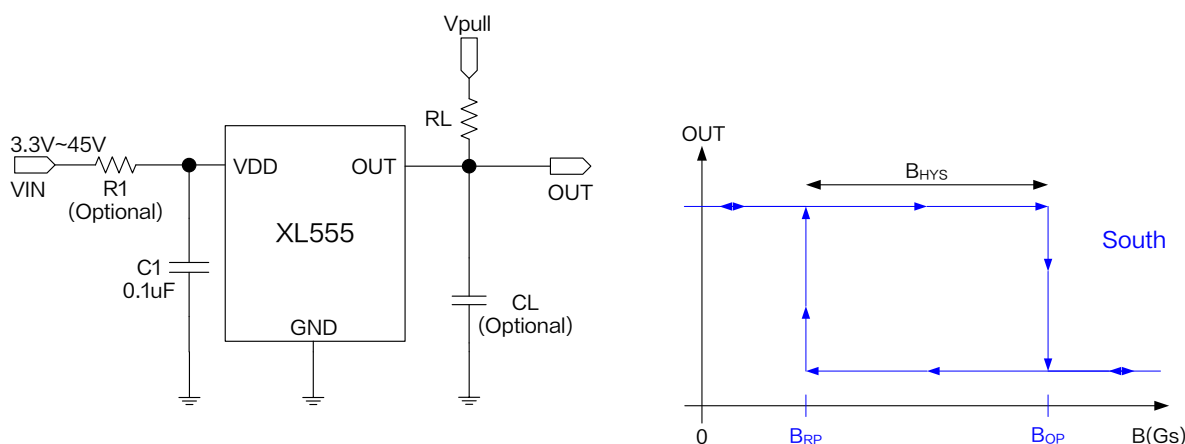
Figure1. XL555 Typical application schematic and output characteristic curve
