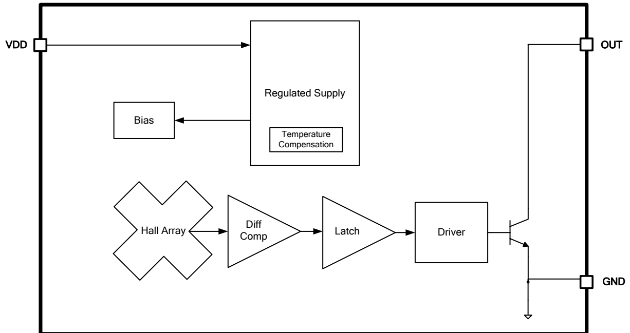
Figure3. Function Block Diagram of XL555
