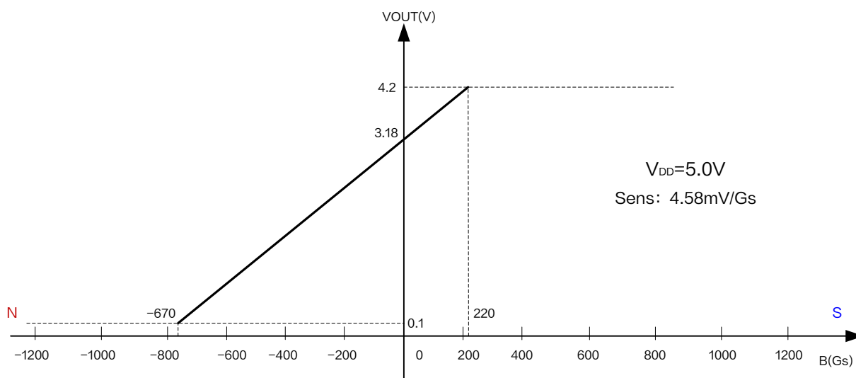
Figure6.XL47 Output characteristic curve ( V_{DD} = 5.0V )
