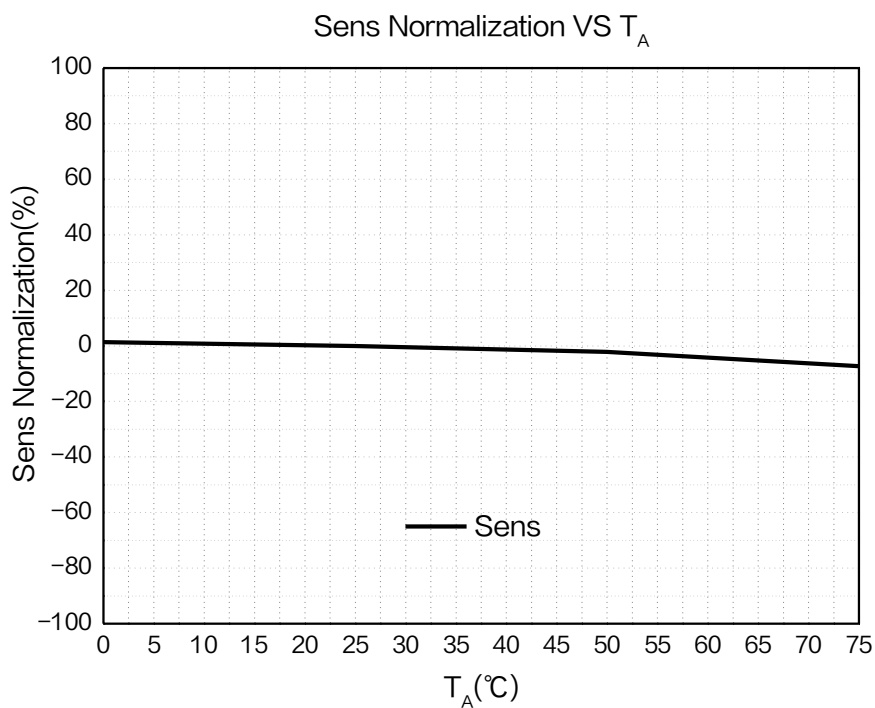
Figure7.Sensitivity versus temperature curve of XL47 ( V_{DD} = 3.3V )
