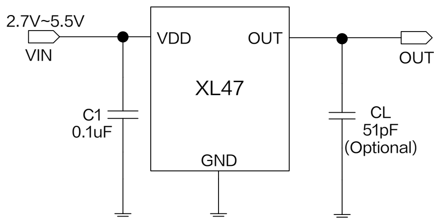
Figure1.XL47 Typical application schematic
