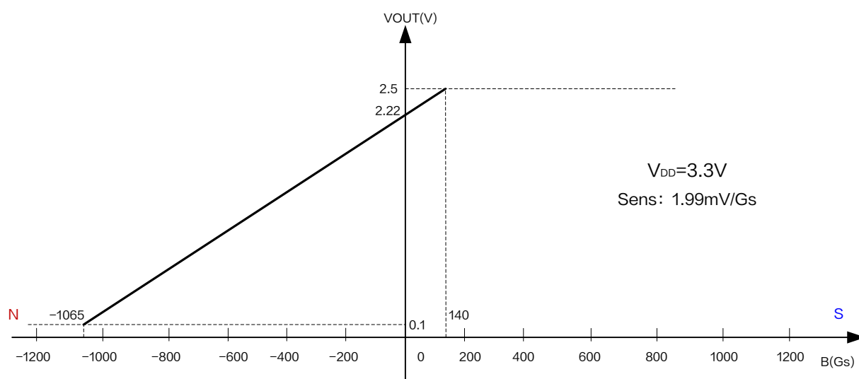
Figure5.XL47 Output characteristic curve ( V_{DD} = 3.3\text{V} )
