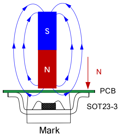
Figure4.Application diagram of XL46
