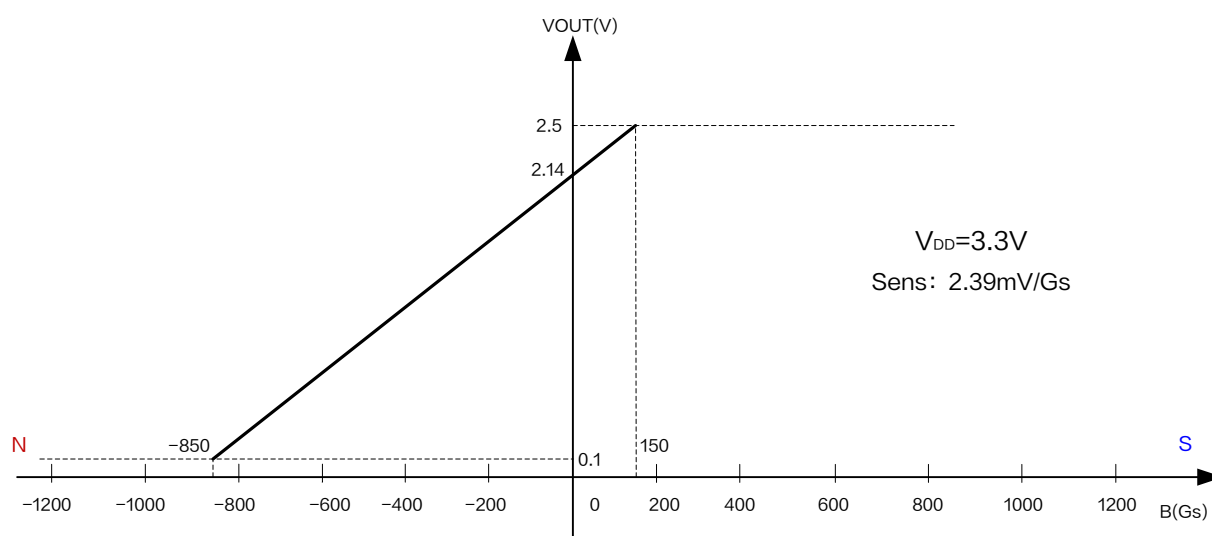
Figure5.XL46 Output characteristic curve ( V_{DD} = 3.3\text{V} )
