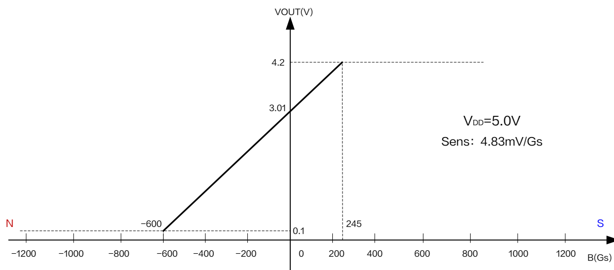
Figure6.XL46 Output characteristic curve ( V_{DD} = 5.0V )
