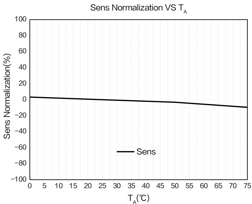
Figure7.Sensitivity versus temperature curve of XL46 ( V_{DD} = 3.3V )
