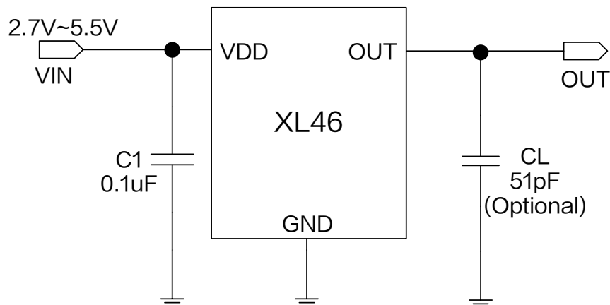
Figure1.XL46 Typical application schematic
