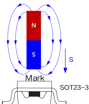
Figure4. Test Schematic of XL44B
