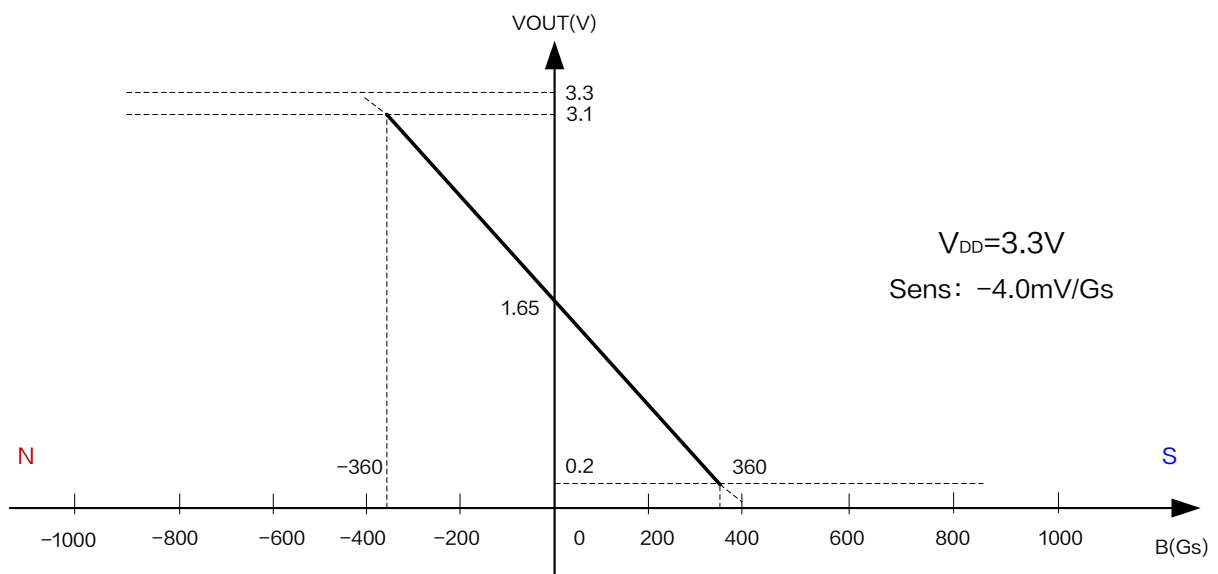
Figure5.Output Characteristic Curve of XL44B ( V_{DD} = 3.3V )
