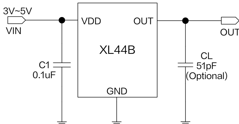
Figure1.XL44B Typical application schematic
