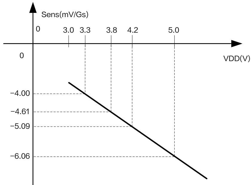
Figure7.Sensitivity Linear Curve of XL44B
