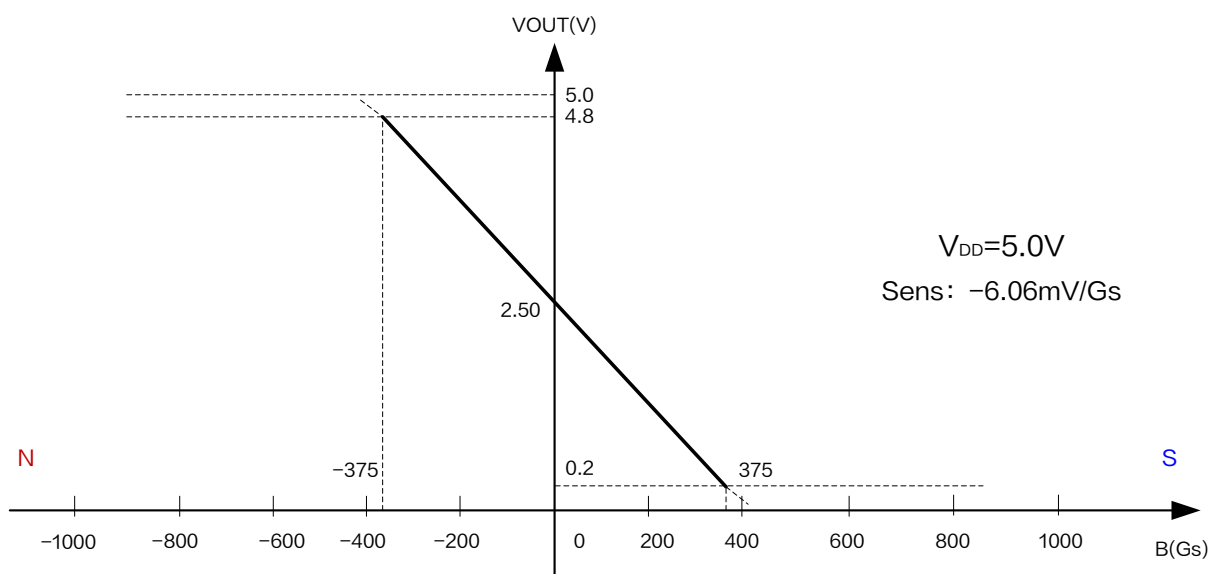
Figure6.Output Characteristic Curve of XL44B ( V_{DD} = 5.0V )
