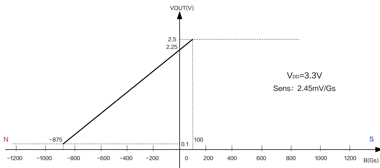
Figure5.XL42P Output characteristic curve ( V_{DD} = 3.3\text{V} )
