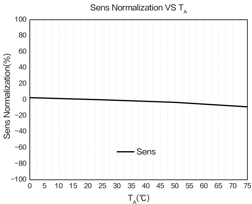
Figure7.Sensitivity versus temperature curve of XL42P ( V_{DD} = 3.3V )
