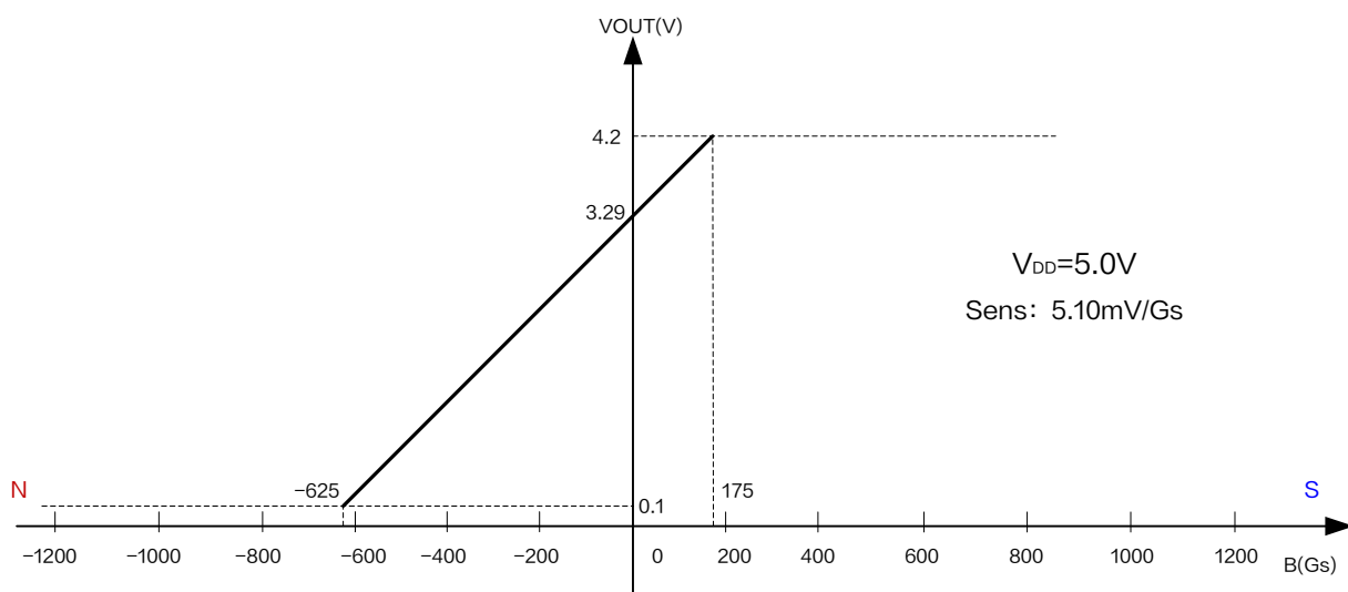
Figure6.XL42P Output characteristic curve ( V_{DD} = 5.0V )
