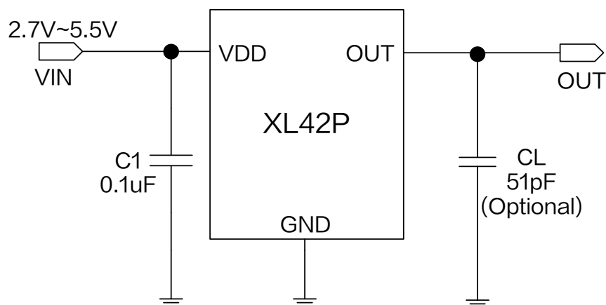
Figure1.XL42P Typical application schematic
